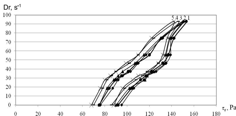
Fig. Rheograms of the gel samples: 1 – after preparation; 2 – in 6 months; 3 – in 12 months; 4 – in 18 months; 5 – in 24 months.
