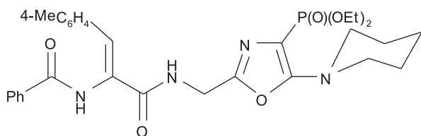
Fig. 1. The chemical formula of diethyl ester of 5-piperidino-2-{N-[N-benzoyl-(4-methylbenzal) glycol] aminomethyl}-1,3-oxazole-4-yl-phosphonic acid
